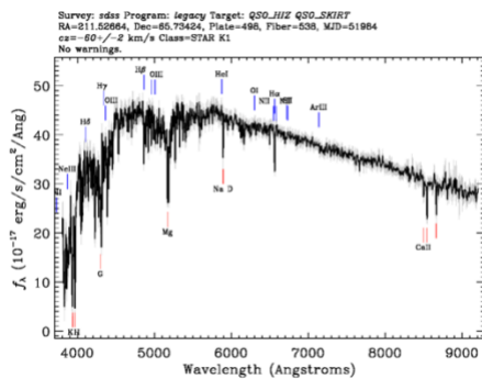
Plate: 498/51984 Fiber: 538
