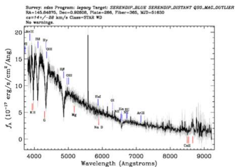
Plate: 266/1630 Fiber: 365
