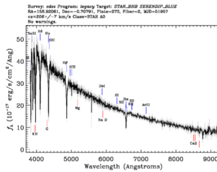
Plate: 273/51597 Fiber: 157
