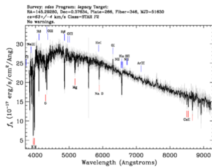
Plate: 266/1630 Fiber: 275
