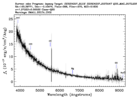
Plate: 266/1630 Fiber: 365
