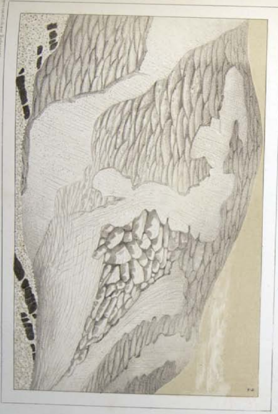
STRATIFICATION OF THE GLACIER OF ST. PIERRE
