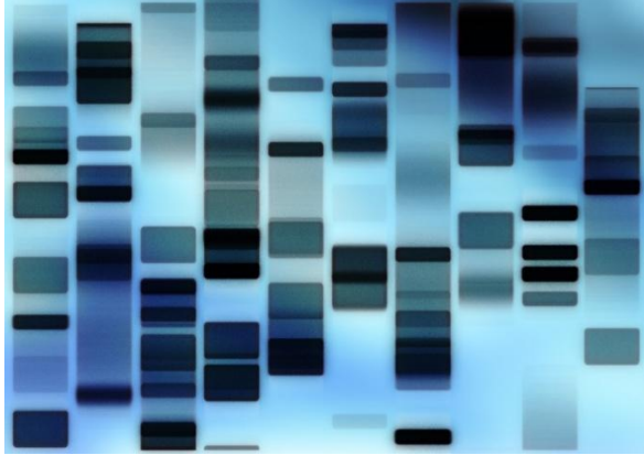
Gel Electrophoresis
