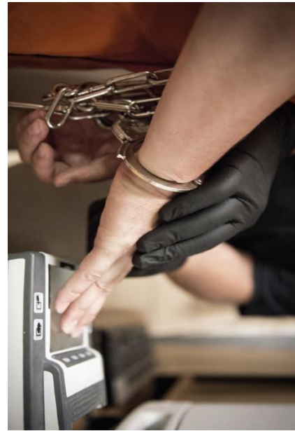
Fingerprinting
